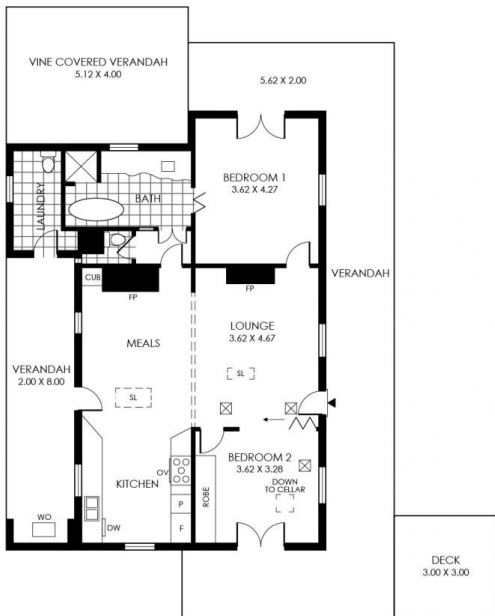
GROUND LEVEL
