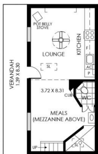
GROUND LEVEL
